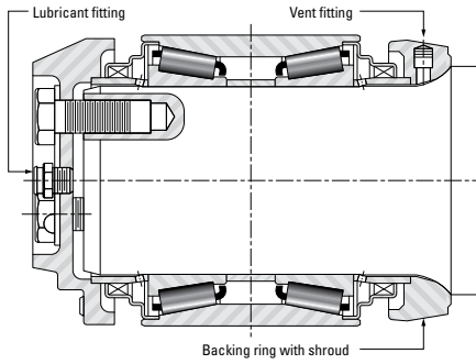
Fig. 34 Mounting Arrangement 1
