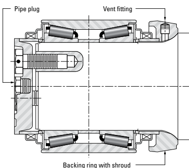
Fig. 49 Mounting Arrangement 6
