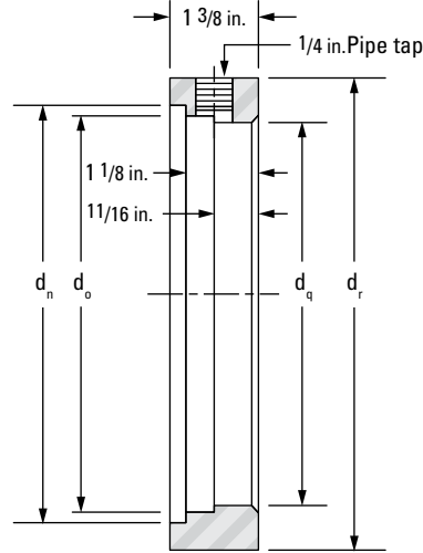
Backing Spacer
